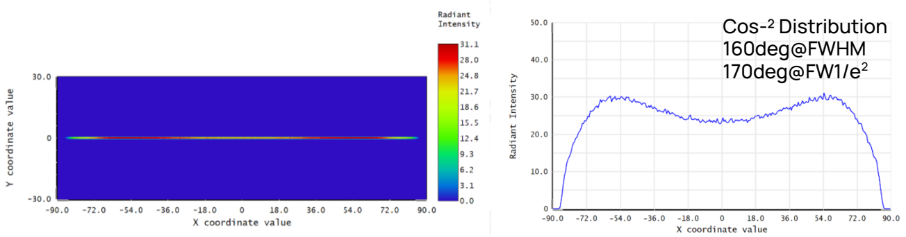
Angular Distribution Pattern (Left) and Angular Output Profile (Right)
