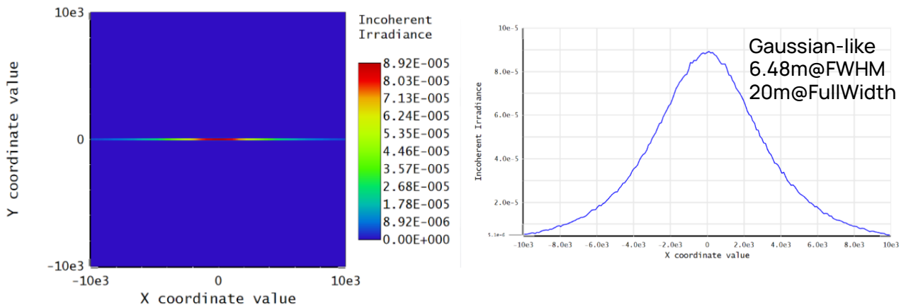
Spatial Distribution Pattern (Left) and Spatial Output Profile (Right), 1 meter away from Diffuser
